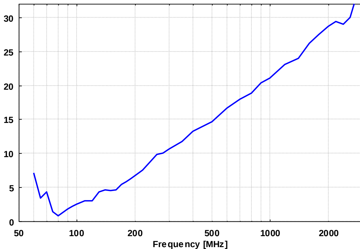
Antenna Factor STLP 9128 E
