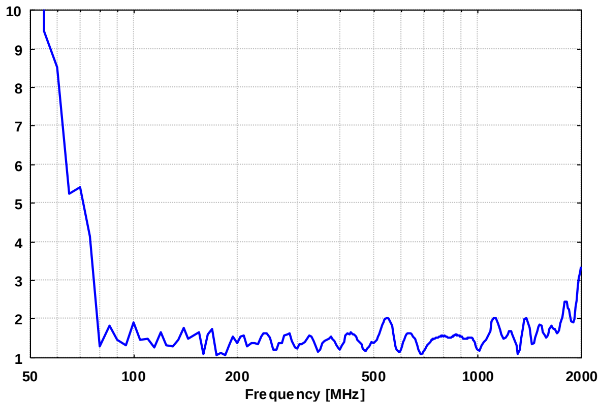
Individual SWR-Plot STLP 9128 E
