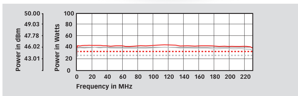
Power amplifier of NSG 4070C2-35
