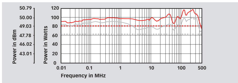
Power amplifier of NSG 4070C2-60
