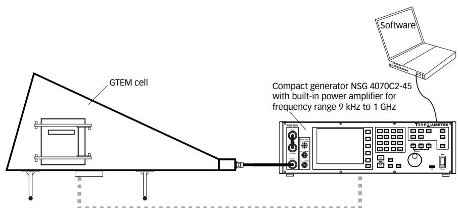
Application for IEC / EN 61000-4-20 up to 1 GHz (example with NSG 4070C2-45; field probe control requires optional software e.g. CIS)
