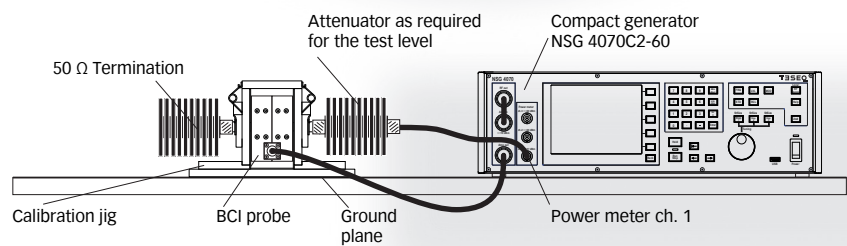
Application for automotive BCI, calibration set-up (example with NSG 4070C2-60)
