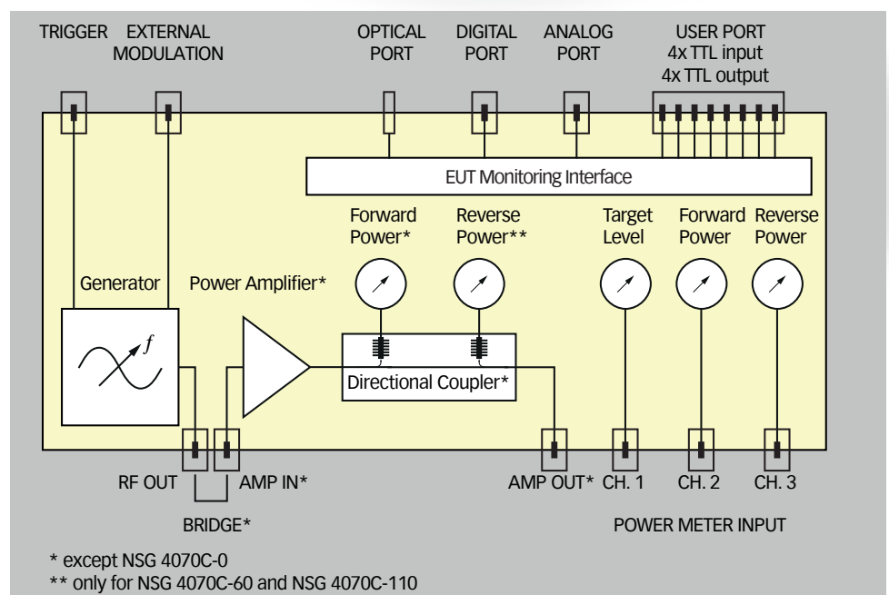
Block diagram of NSG 4070C2
