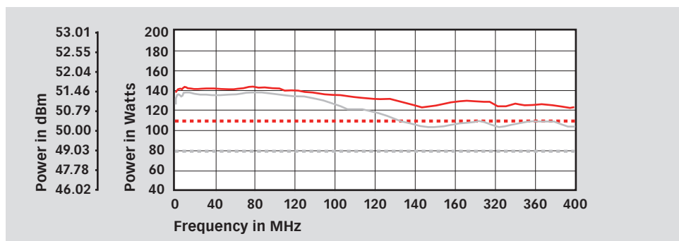
Power amplifier of NSG 4070C2-110
