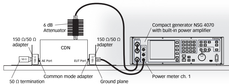
Application for IEC / EN 61000-4-6, calibration set-up with CDN
