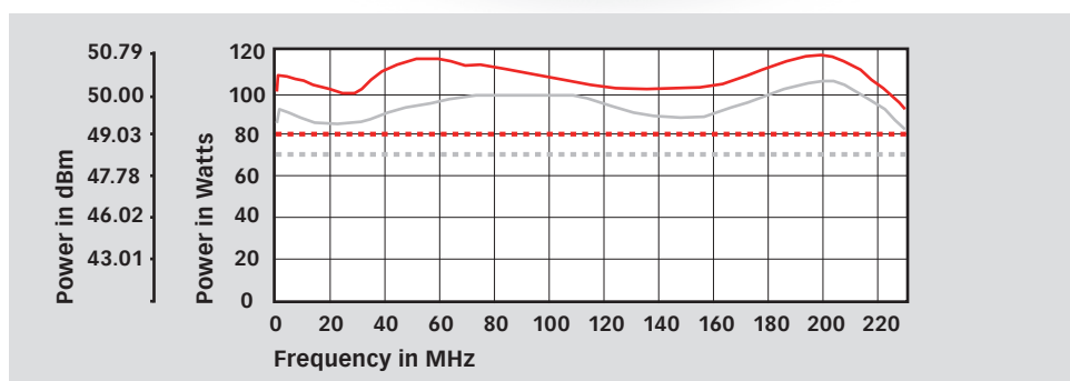
Power amplifier of NSG 4070C2-80
