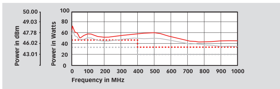
Power amplifier of NSG 4070C2-45
