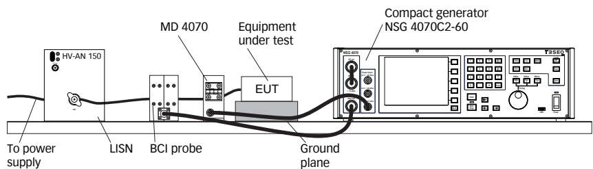
Application for automotive BCI, EUT set-up with monitoring probe and LISN (example with NSG 4070C2-60)
