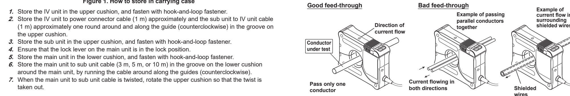
Figure 2. Feed-through example
