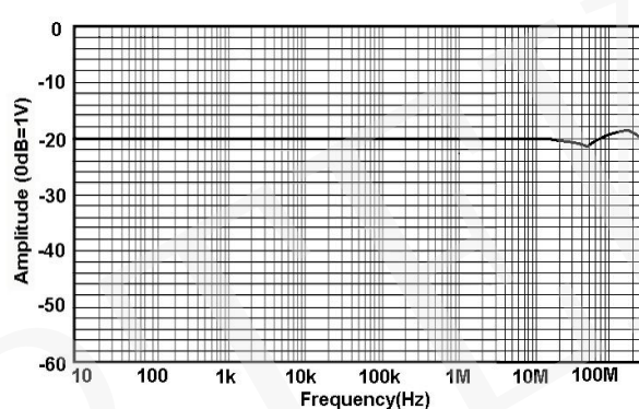
Fig 1 .d HCP8030H Amp- Frequency curve
