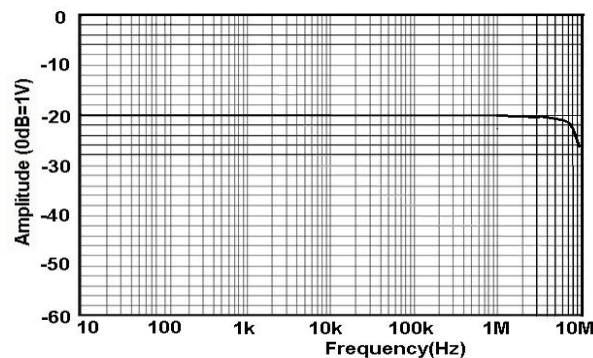
Fig 13.b HCP8300A Amplitude-frequency Curve
