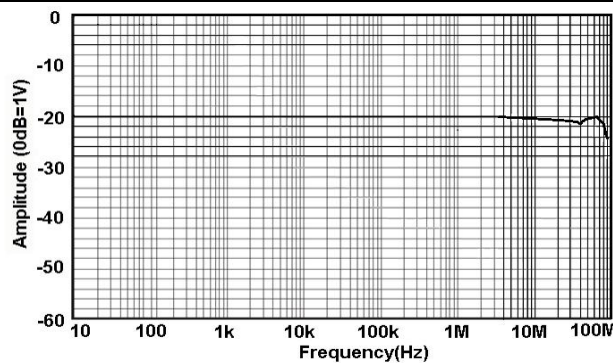
Fig 1 .b HCP8030C Amp- Frequency curve
