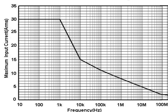
Fig.2.d HCP8030H Continuous maximum input measurement
