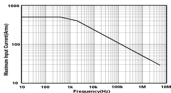
Fig 17 HCP8500 Maximum continuous input measurement
