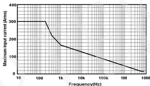
Fig 14.b HCP8300A Continuous maximum input measurement
