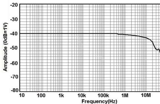
Fig 13.a HCP8300 Amplitude-frequency Curve
