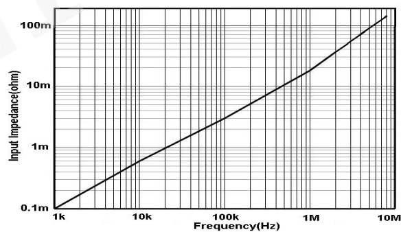
Fig 15.b HCP8300A Input Impedance-Frequency Curve
