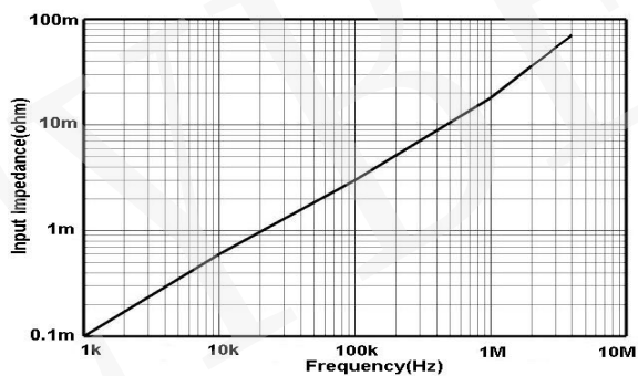
Fig 15.a HCP8300 Input Impedance-Frequency Curve
