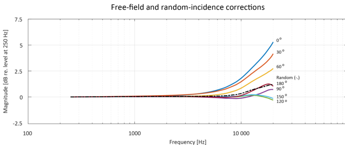
Free-field corrections for different angles of incidence with grid
