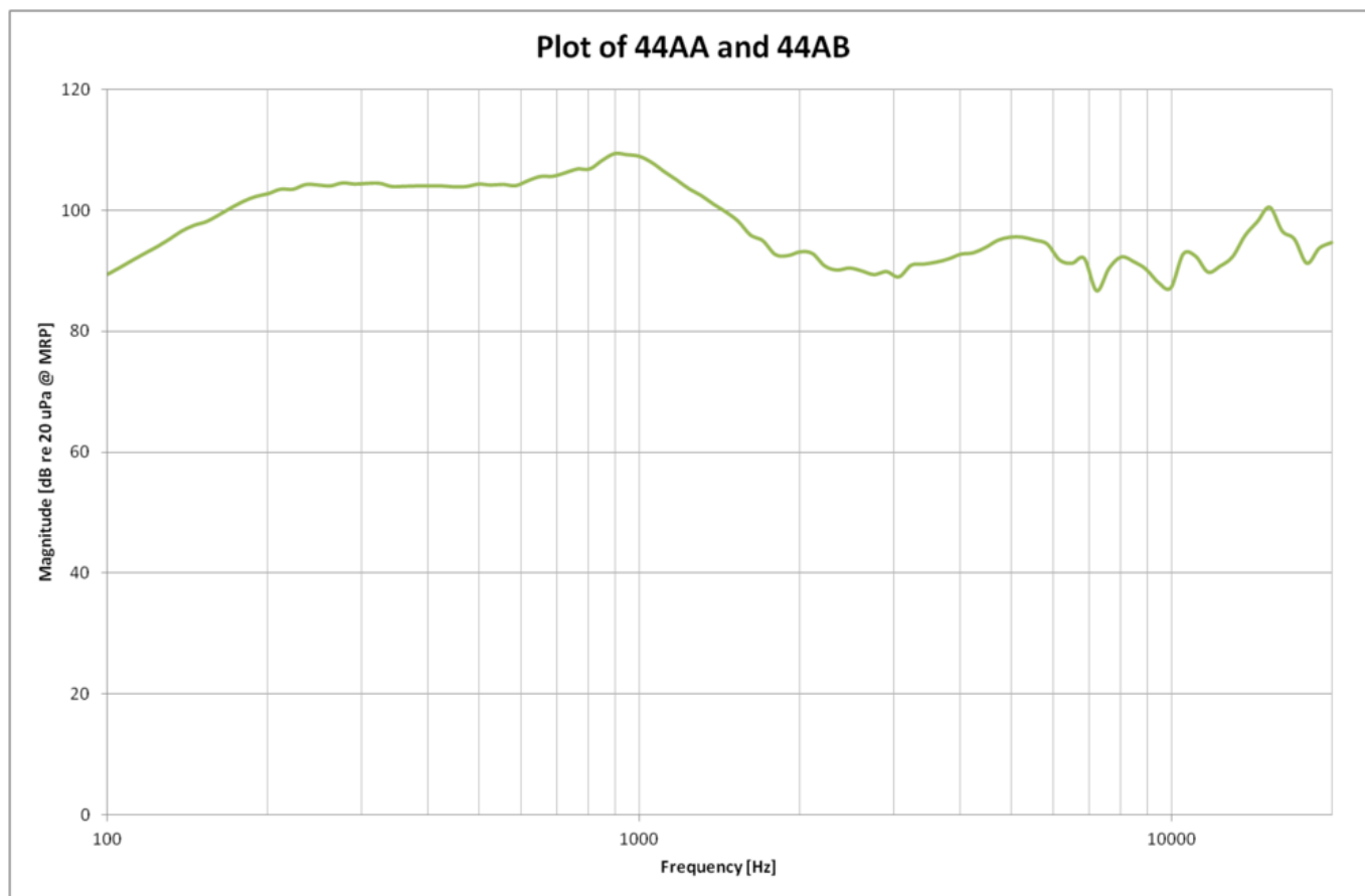
Frequency response
