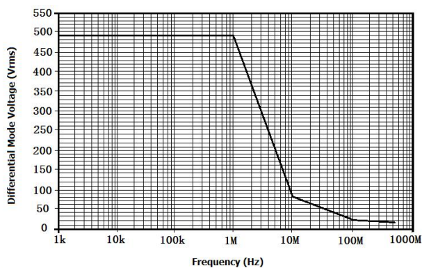
Figure 1:DP6070B Differential Mode Voltage VS Frequency
