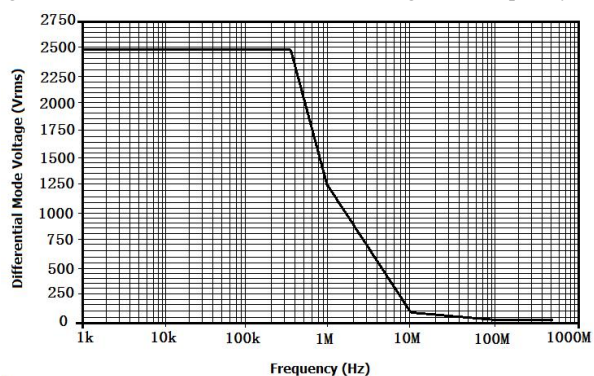
Figure 3:DP6350B Differential Mode Voltage VS Frequency
