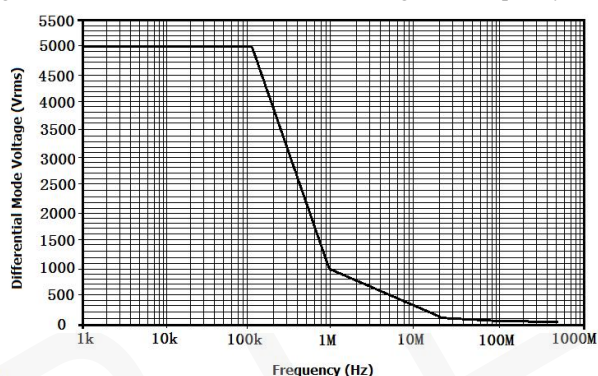
Figure 4:DP6700B Differential Mode Voltage VS Frequency
