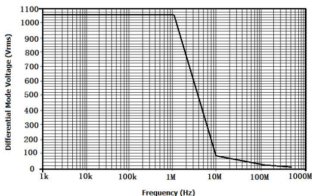
Figure 2:DP6150B Differential Mode Voltage VS Frequency
