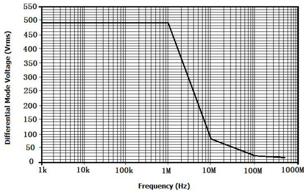
Figure 1:DP6070A Differential Mode Voltage VS Frequency
