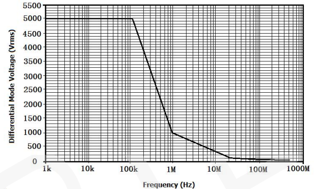
Figure 4:DP6700A Differential Mode Voltage VS Frequency
