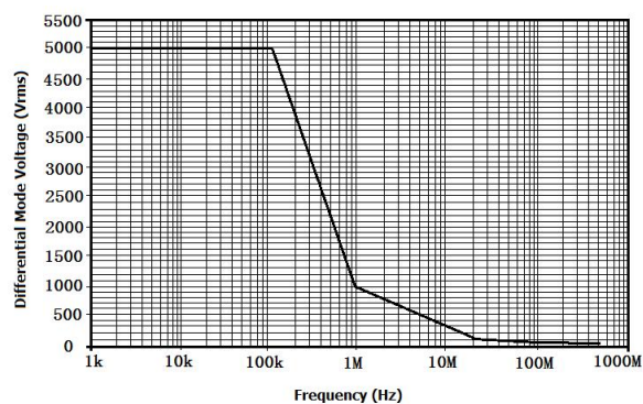
Figure 3:DP6700 Differential Mode Voltage VS Frequency
