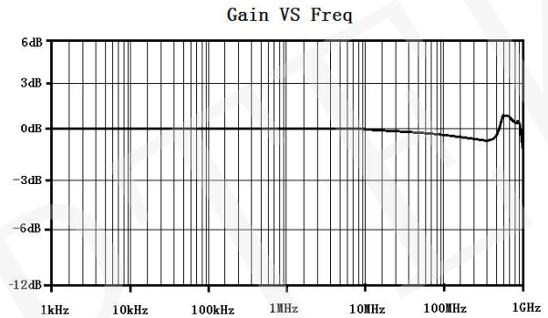
Fig 3: DP6060B Frequency Response Curve
