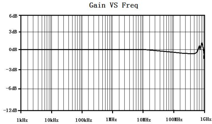
Fig 1: DP6020B Frequency Response Curve
