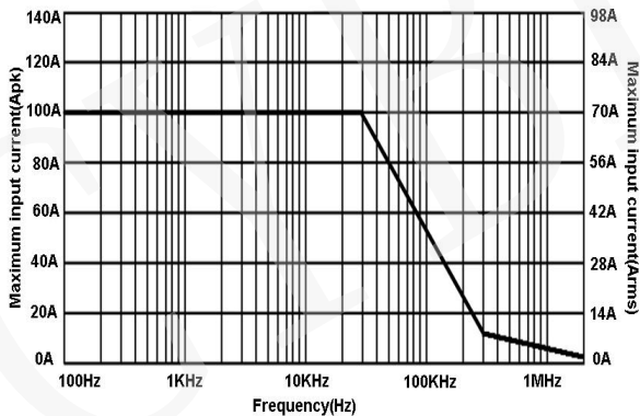
Figure 3 Max current VS Frequency curve
