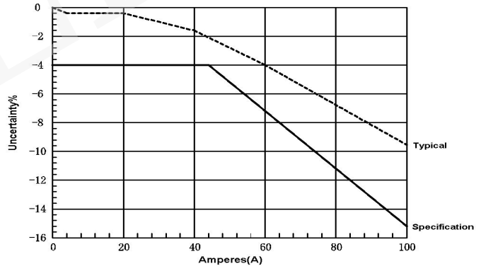
Figure 4 Typical DC linearity (0.01V/A level)
