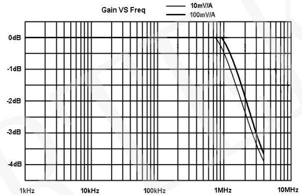
Figure 2 CPL8100B Typical Gain VS Frequency curve
