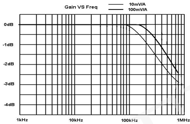
Figure 1 CPL8100A Typical Gain VS Frequency curve
