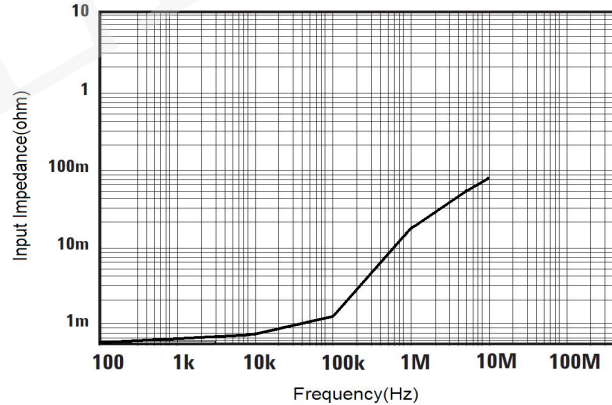
Figure 21 CP4040 insertion loss vs frequency curve
