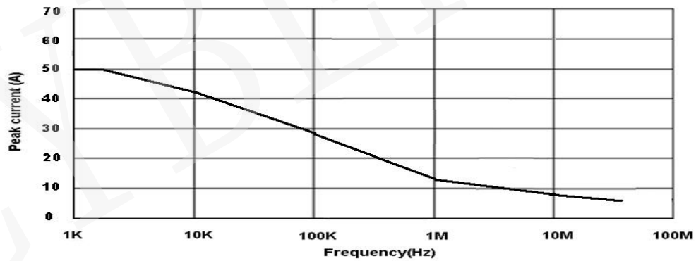
Figure 15 CP3050 Maximum Peak Value Current vs Frequency Curve
