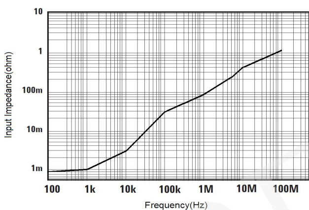
Figure 18 CP3120 insertion loss vs frequency curve
