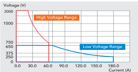
62450D-2000HL Operating Region in Source Mode
