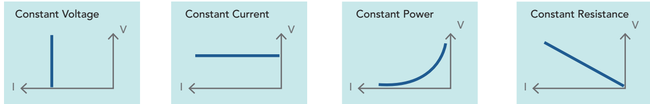
Electrical load functions
